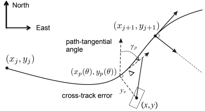
Fig. 1. LOS guidance geometry.
